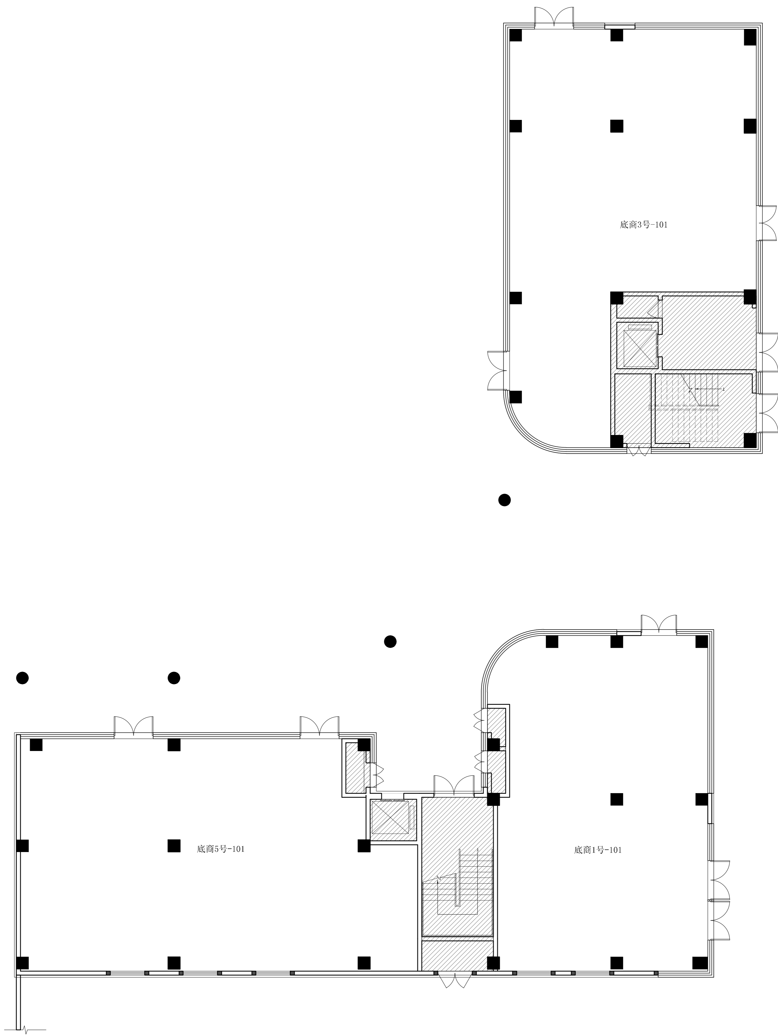
首层平面图 (层高约5.4m)
